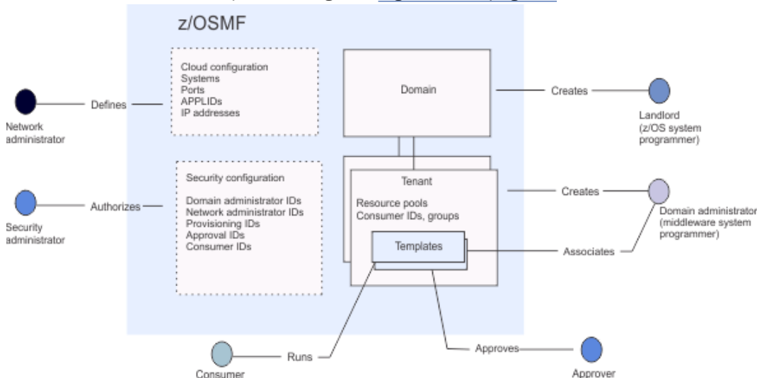
Figure 21. Cloud Provisioning Summary
