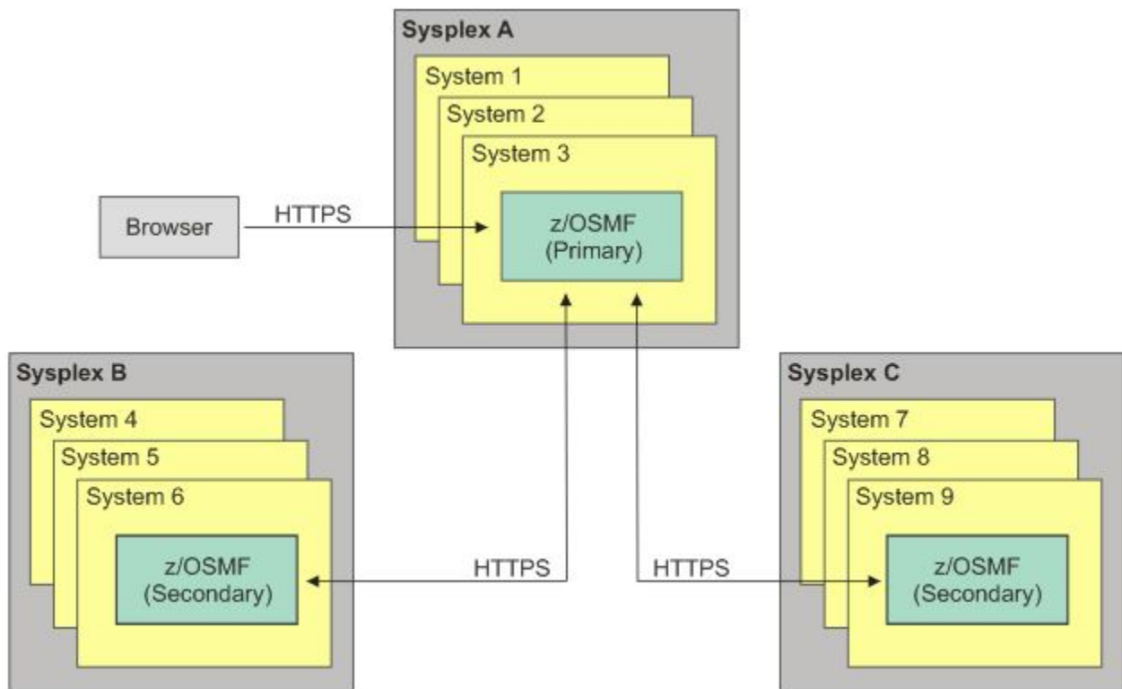
Figure 127. Example sysplex and system configuration
